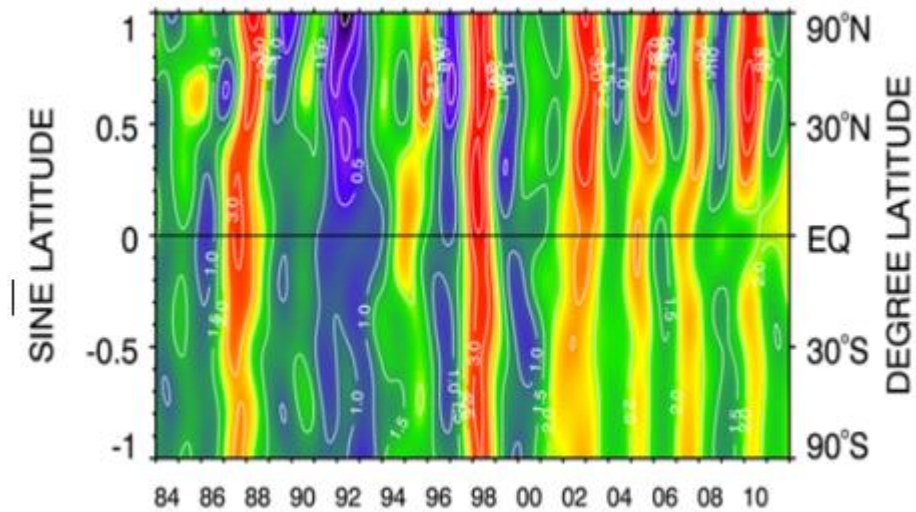
Figure 1 (b): The Change Rate of \text{CO}_2 Concentration (Ppm/Year) Across Latitudes between 1984 and 2011 [11]
