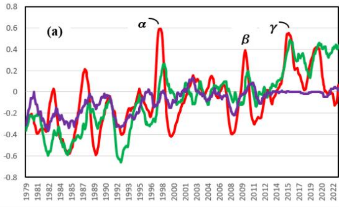
Figure 2(a): Temperature Change ( ^\circ\text{C} ) between 1979 and 2022 in the Tropics (20 S-20 N, Red), North Latitude (20 N-90 N, Green), and South Latitude (20 S-90 S, Purple)
